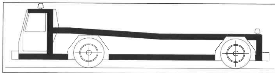
Figure 4: Suggested placement of retroreflective tape on a TLTV
